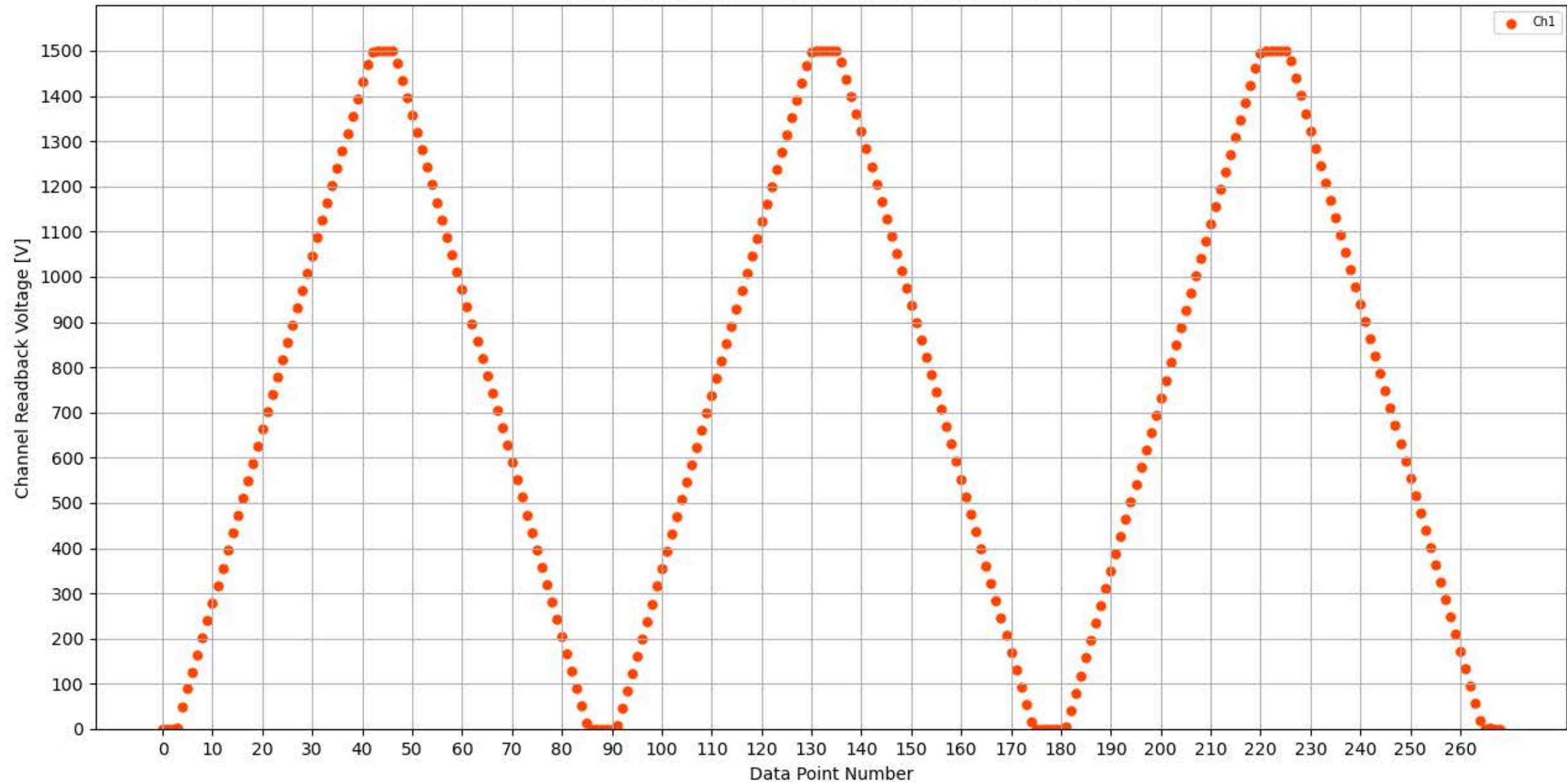
Voltage Ramp Test (Python) Bd #353, Slot #1, Ch #1
