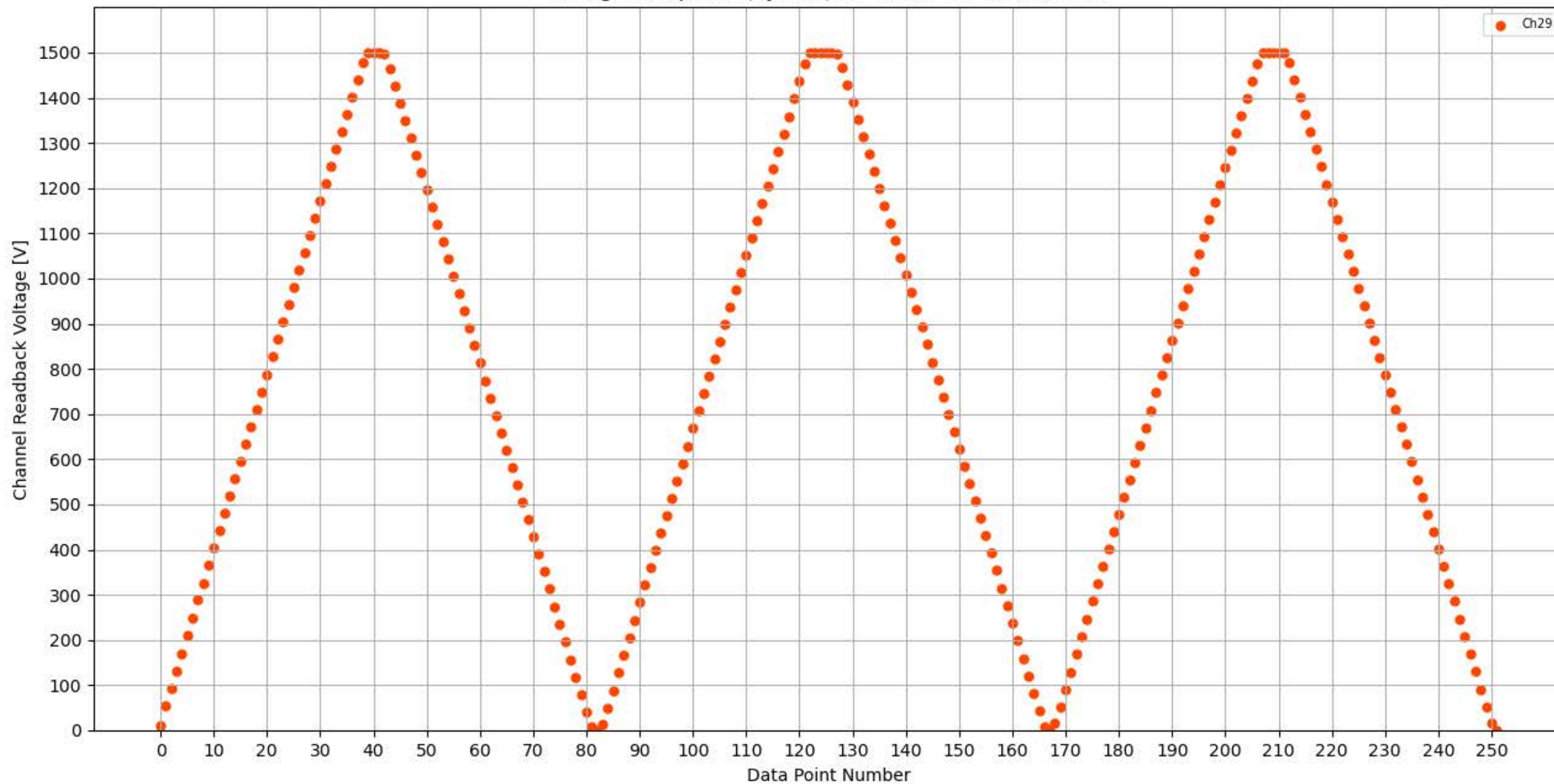
Voltage Ramp Test (Python) Bd #353, Slot #1, Ch #29
