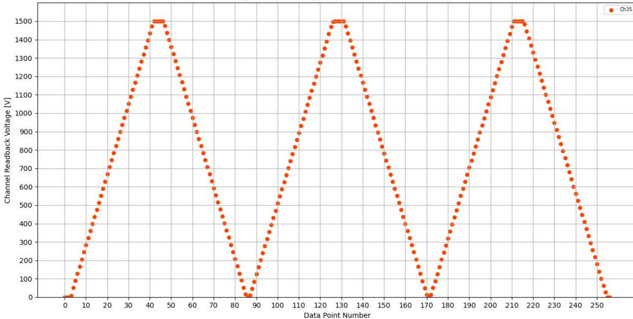
Voltage Ramp Test (Python) Bd #353, Slot #1, Ch #35
