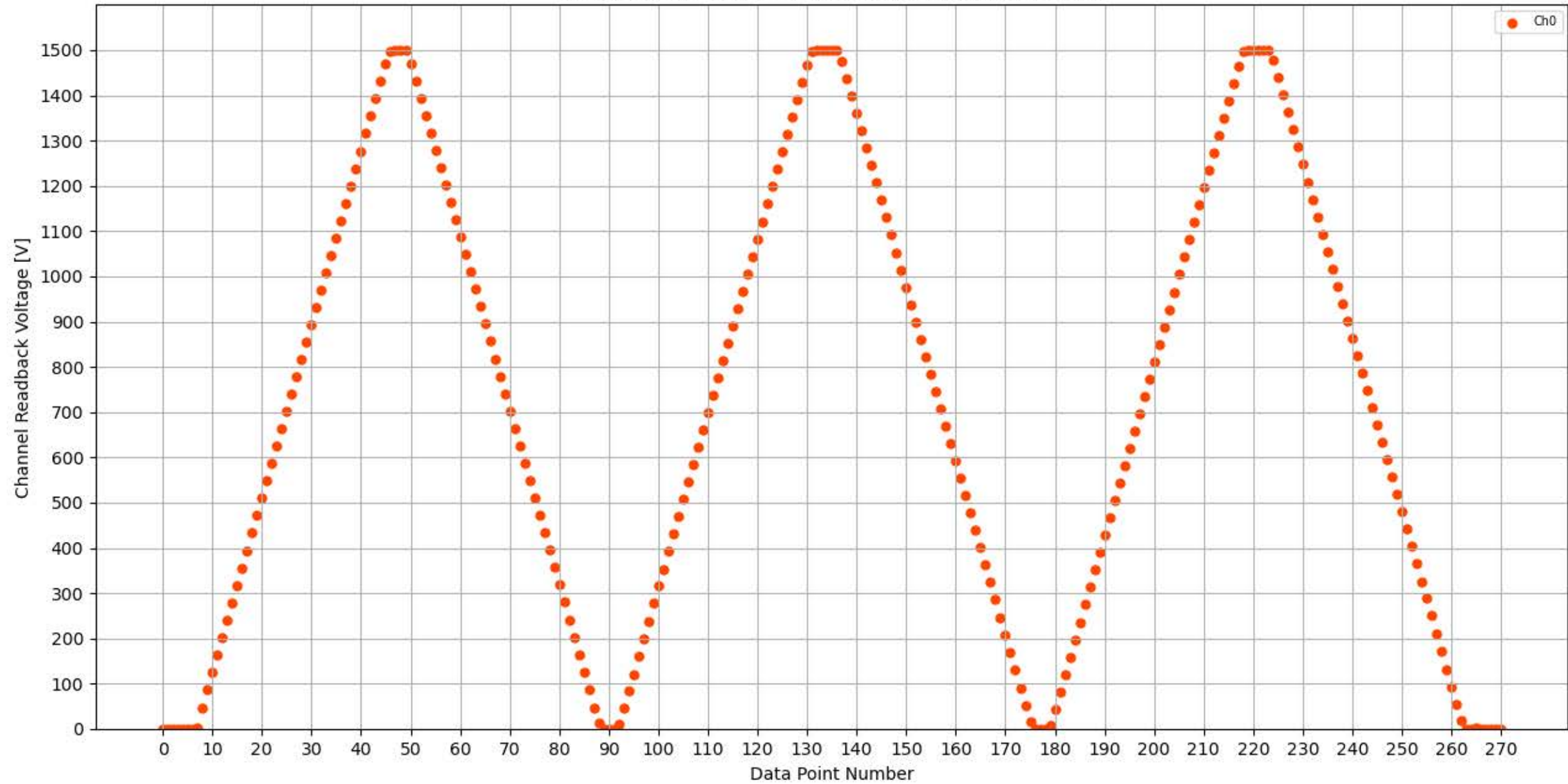
Voltage Ramp Test (Python) Bd #353, Slot #1, Ch #0
