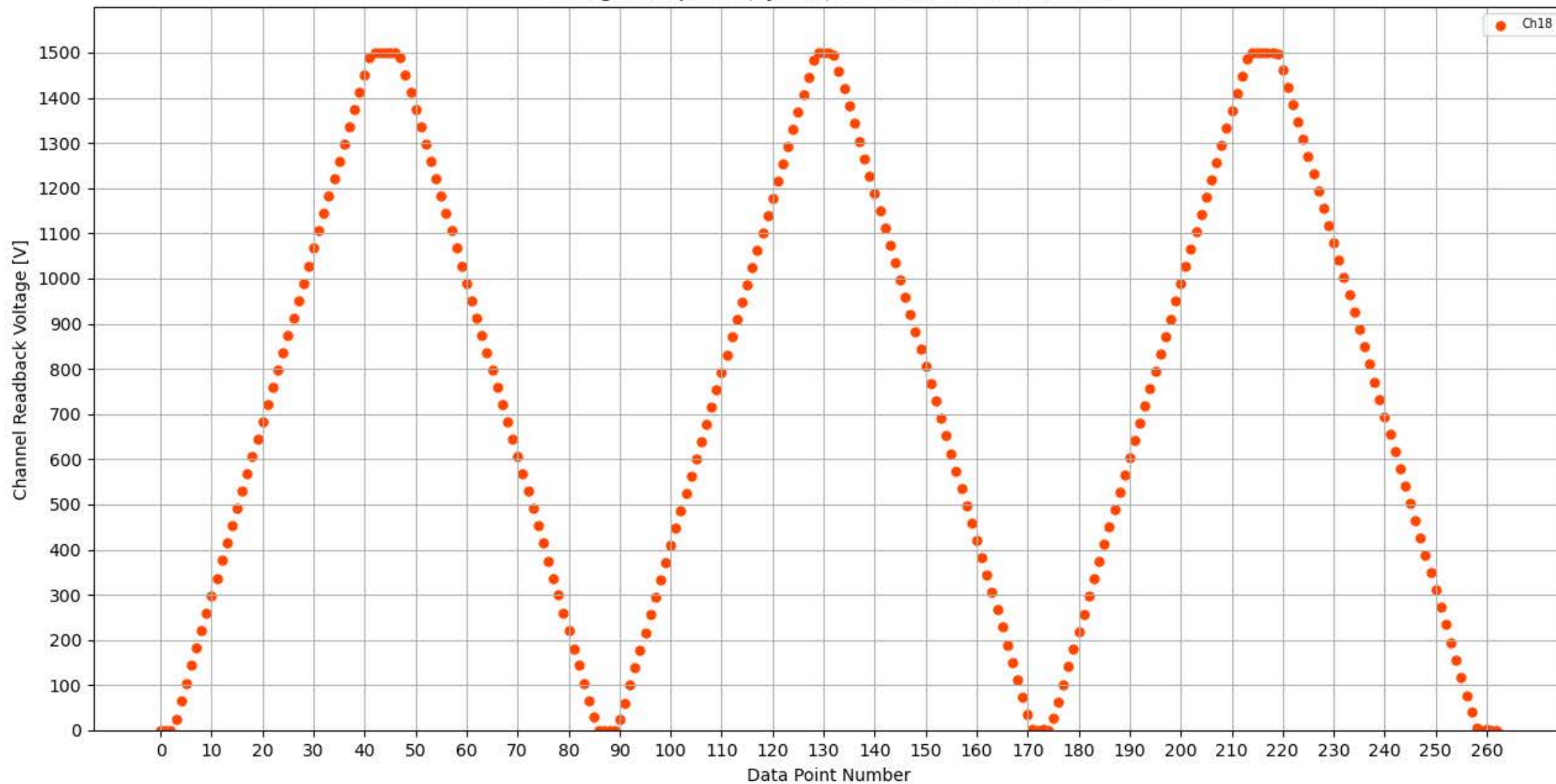
Voltage Ramp Test (Python) Bd #353, Slot #1, Ch #18
