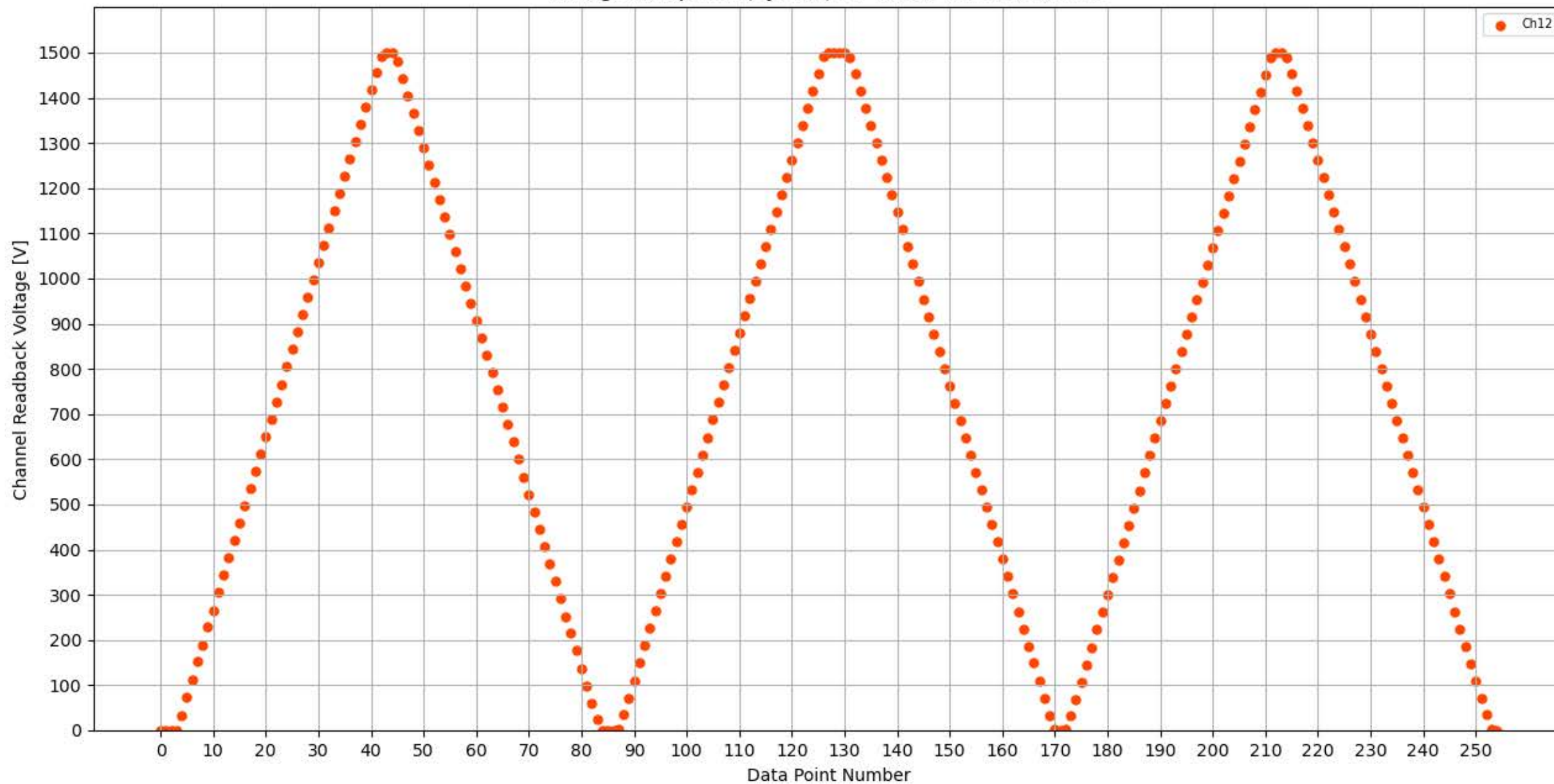
Voltage Ramp Test (Python) Bd #353, Slot #1, Ch #12
