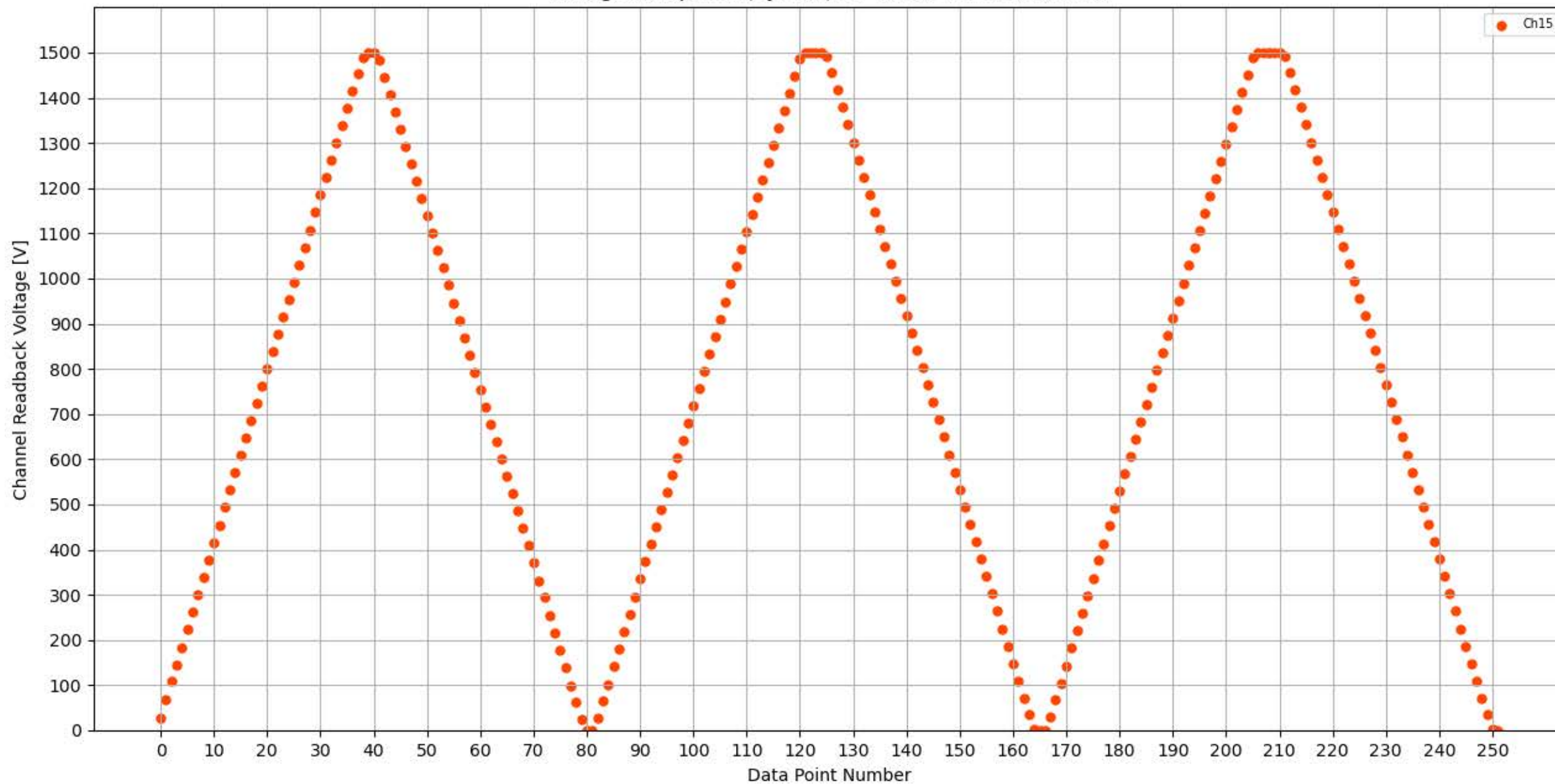
Voltage Ramp Test (Python) Bd #353, Slot #1, Ch #15
