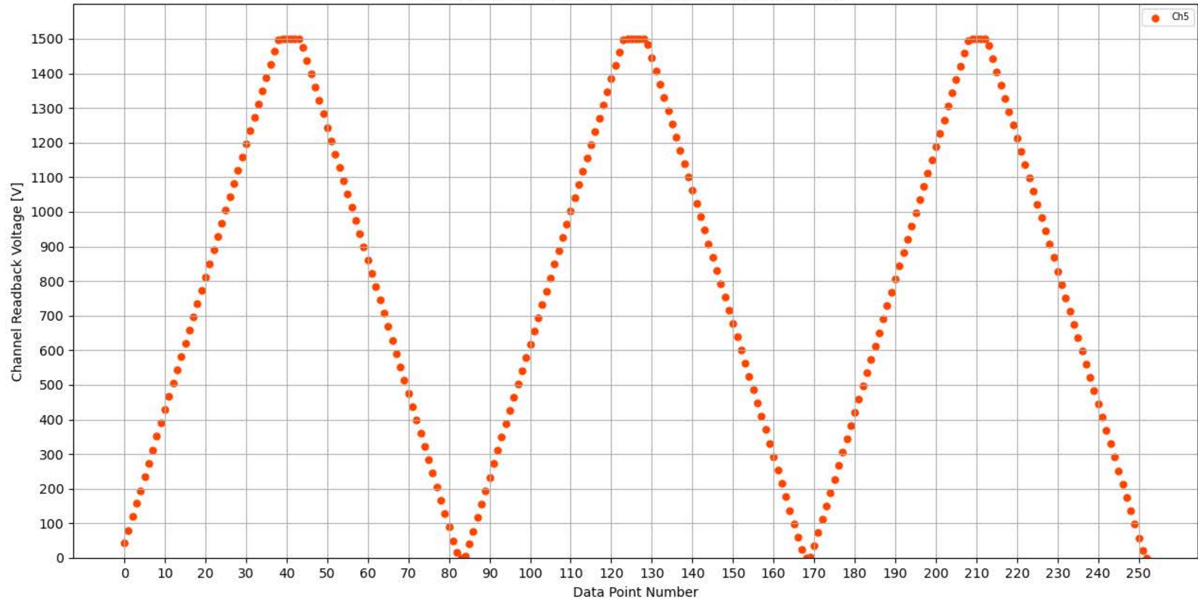
Voltage Ramp Test (Python) Bd #353, Slot #1, Ch #5
