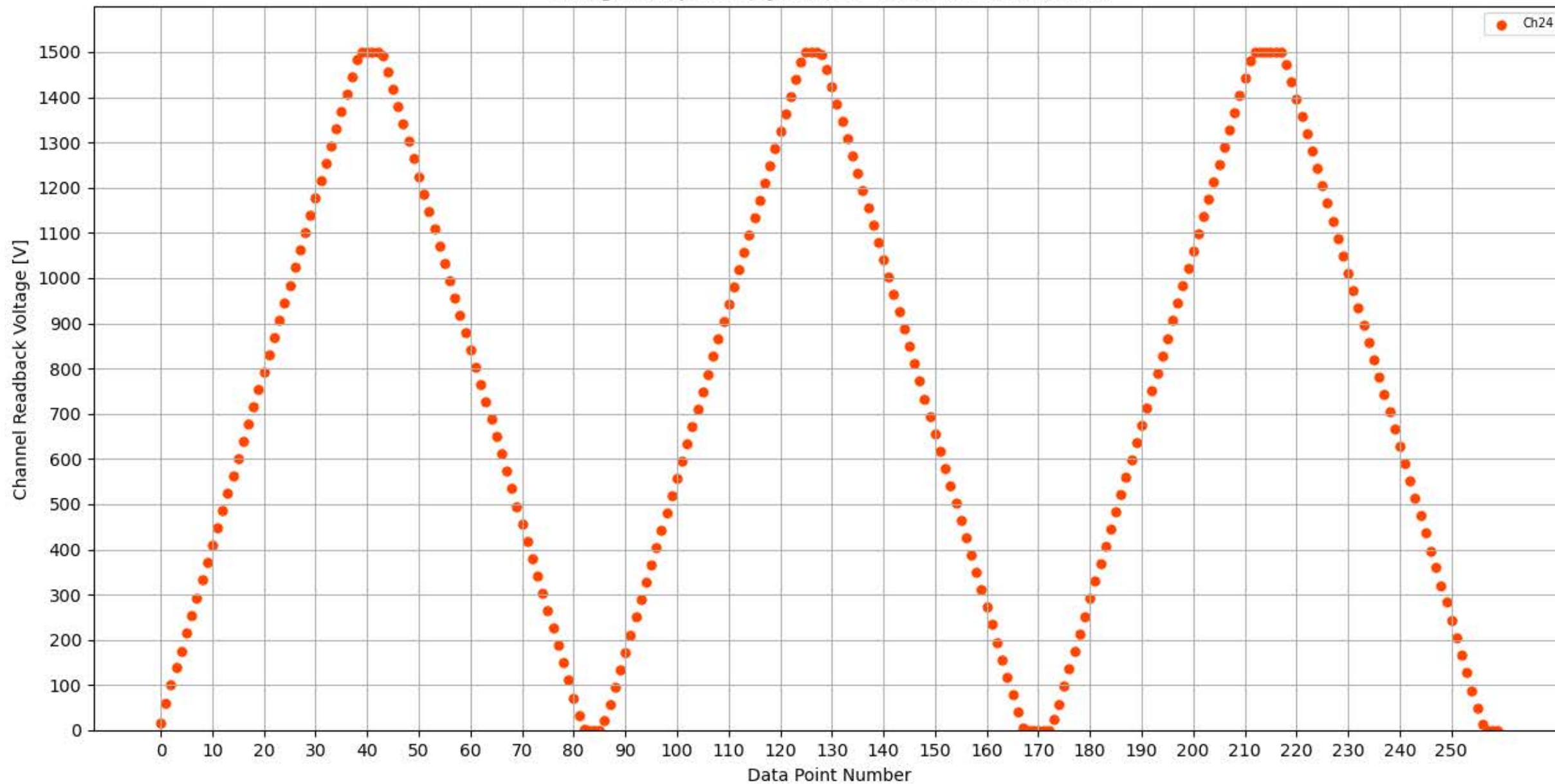
Voltage Ramp Test (Python) Bd #353, Slot #1, Ch #24
