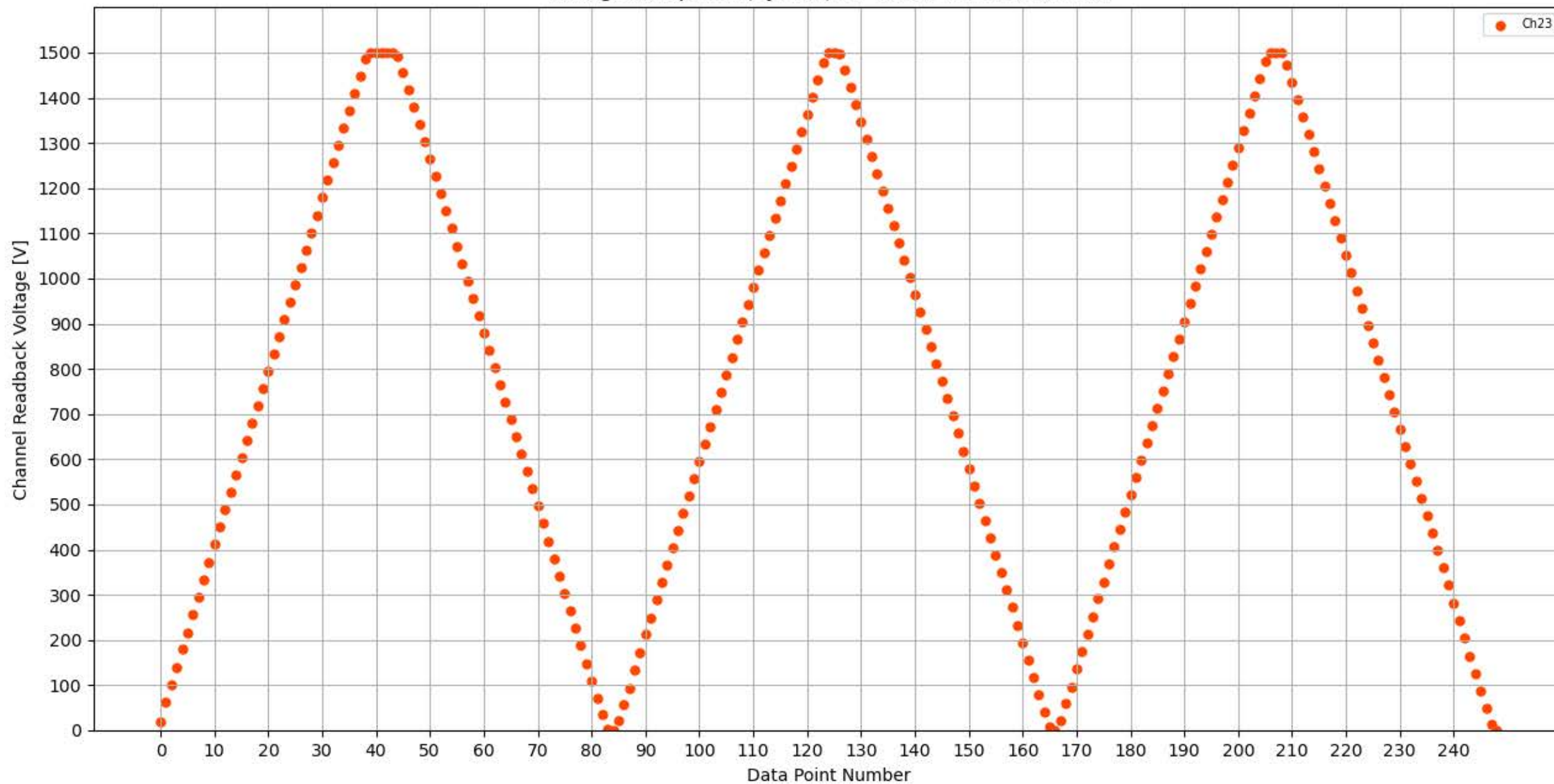
Voltage Ramp Test (Python) Bd #353, Slot #1, Ch #23
