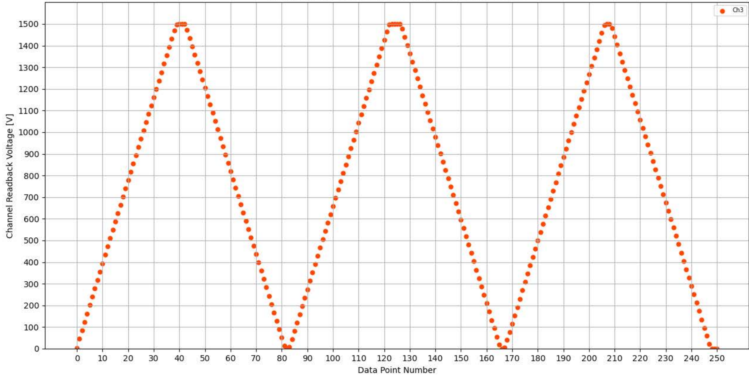
Voltage Ramp Test (Python) Bd #353, Slot #1, Ch #3
