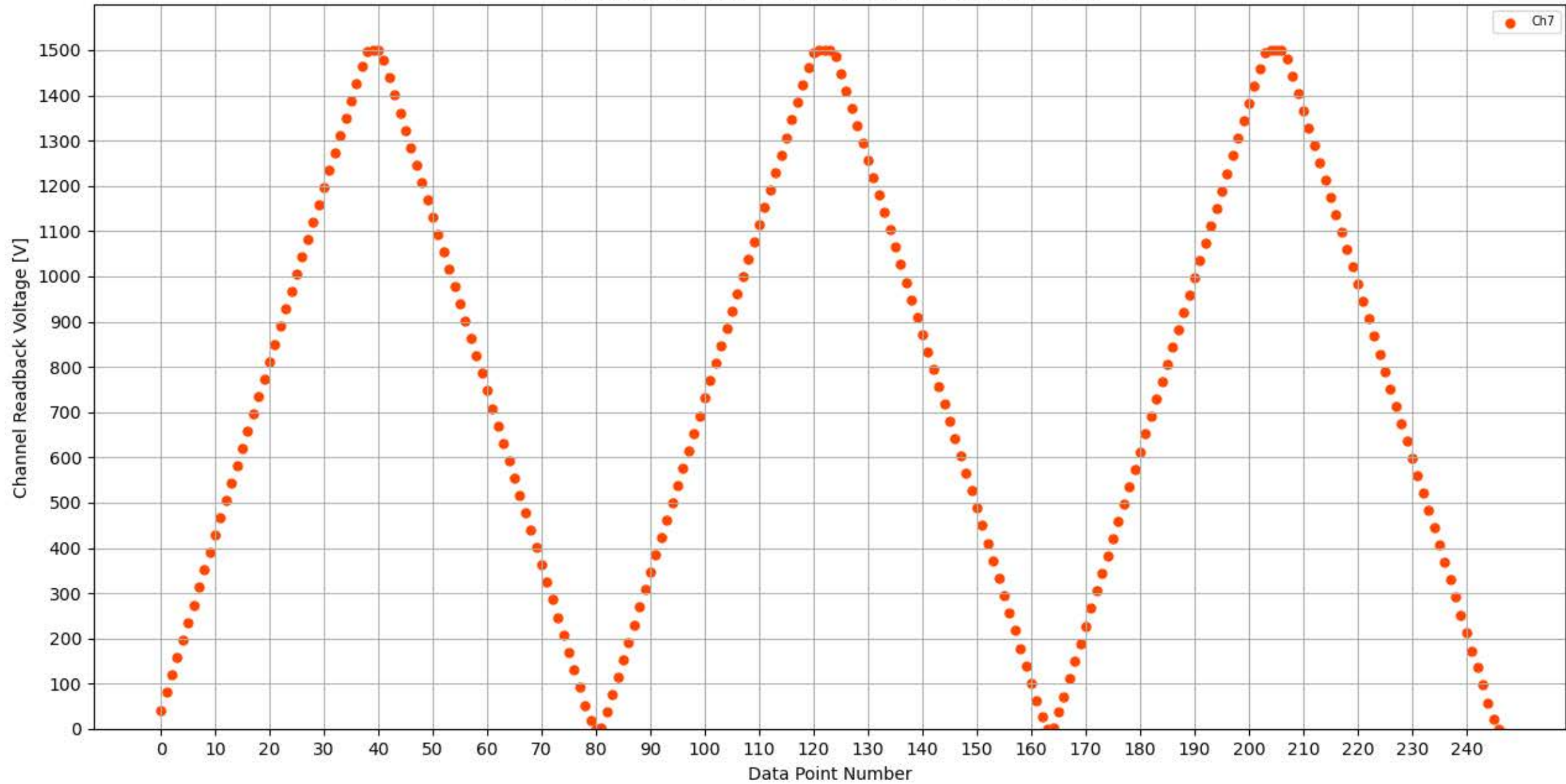
Voltage Ramp Test (Python) Bd #353, Slot #1, Ch #7
