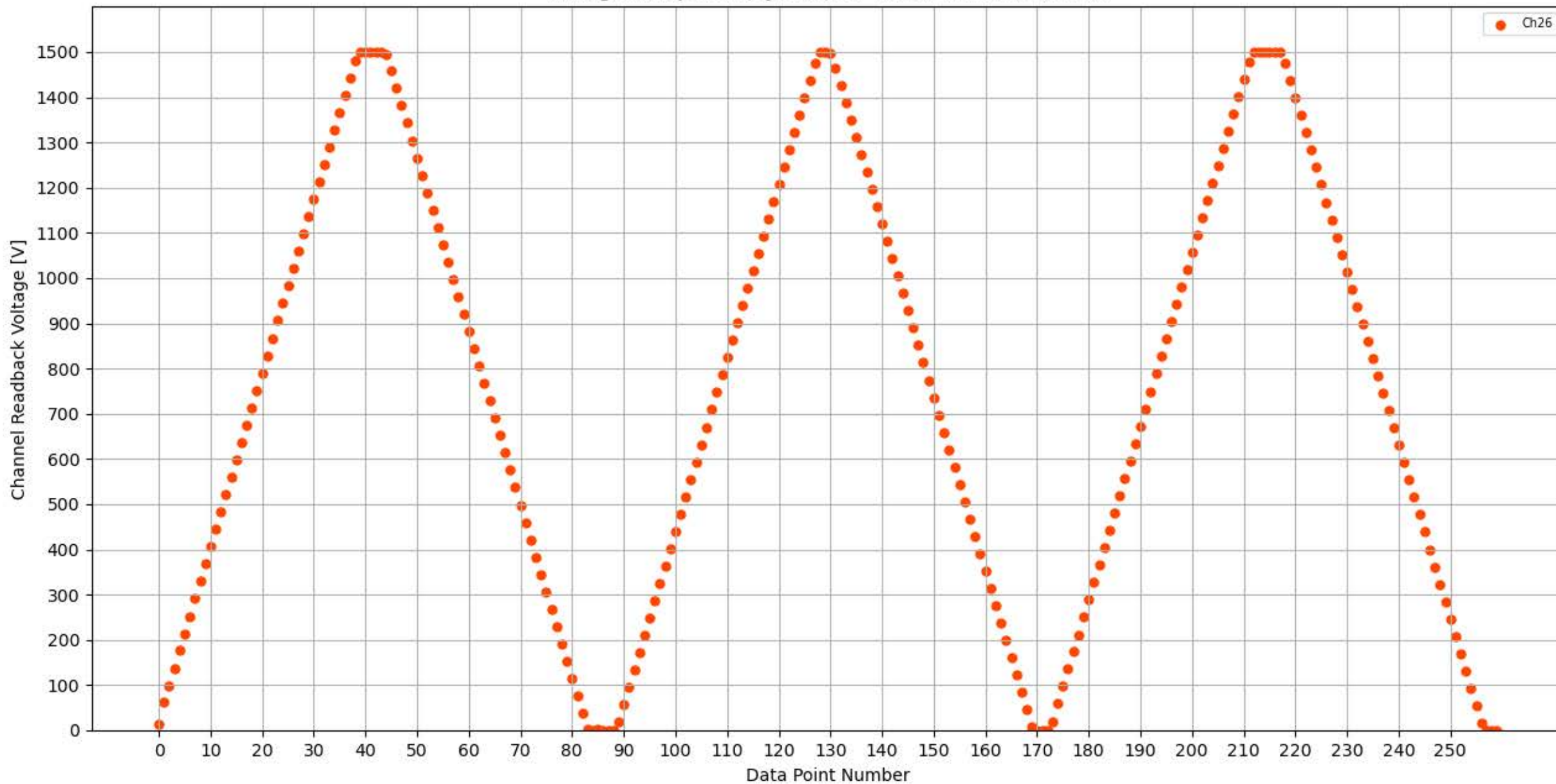
Voltage Ramp Test (Python) Bd #353, Slot #1, Ch #26
