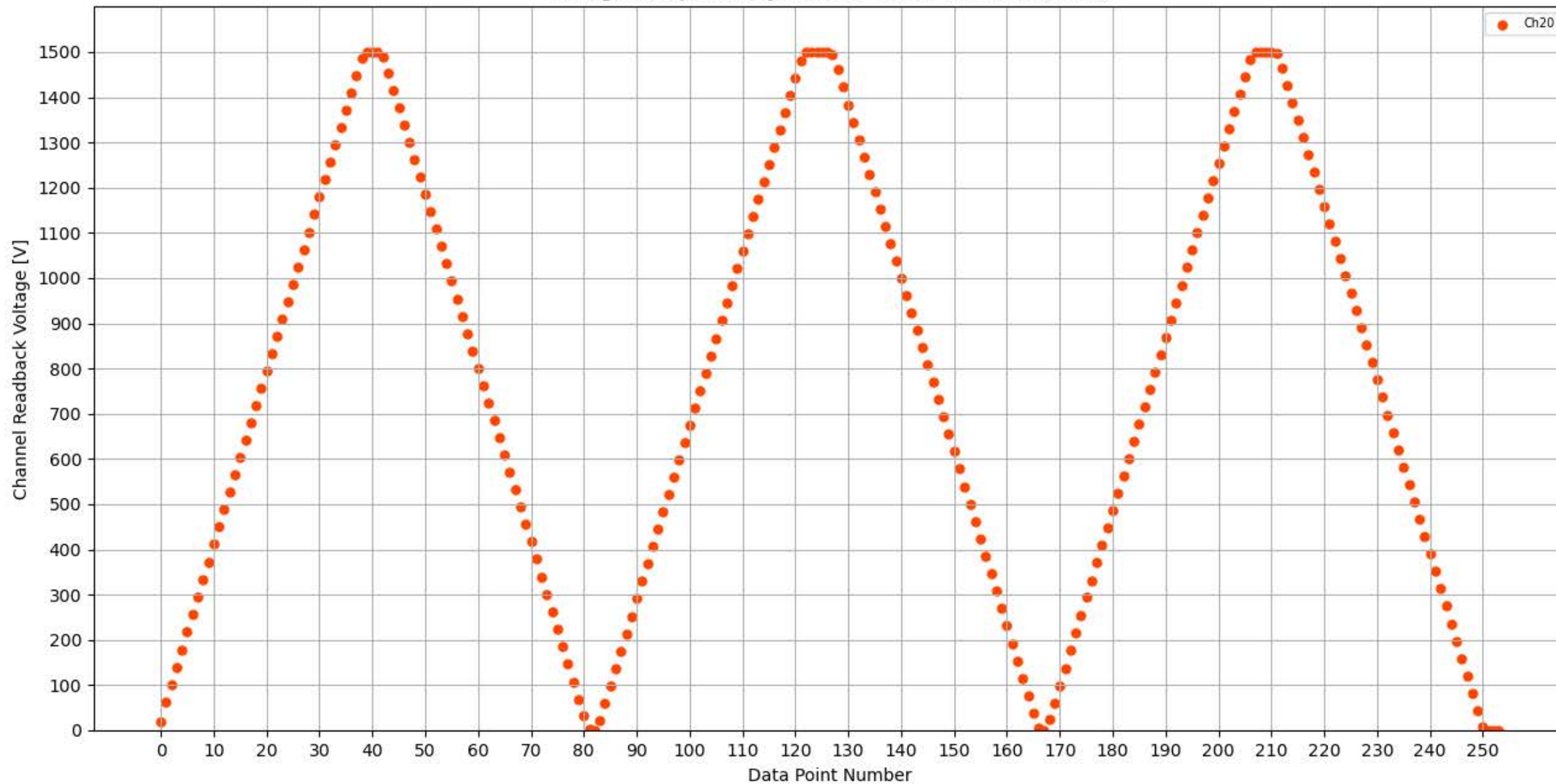
Voltage Ramp Test (Python) Bd #353, Slot #1, Ch #20
