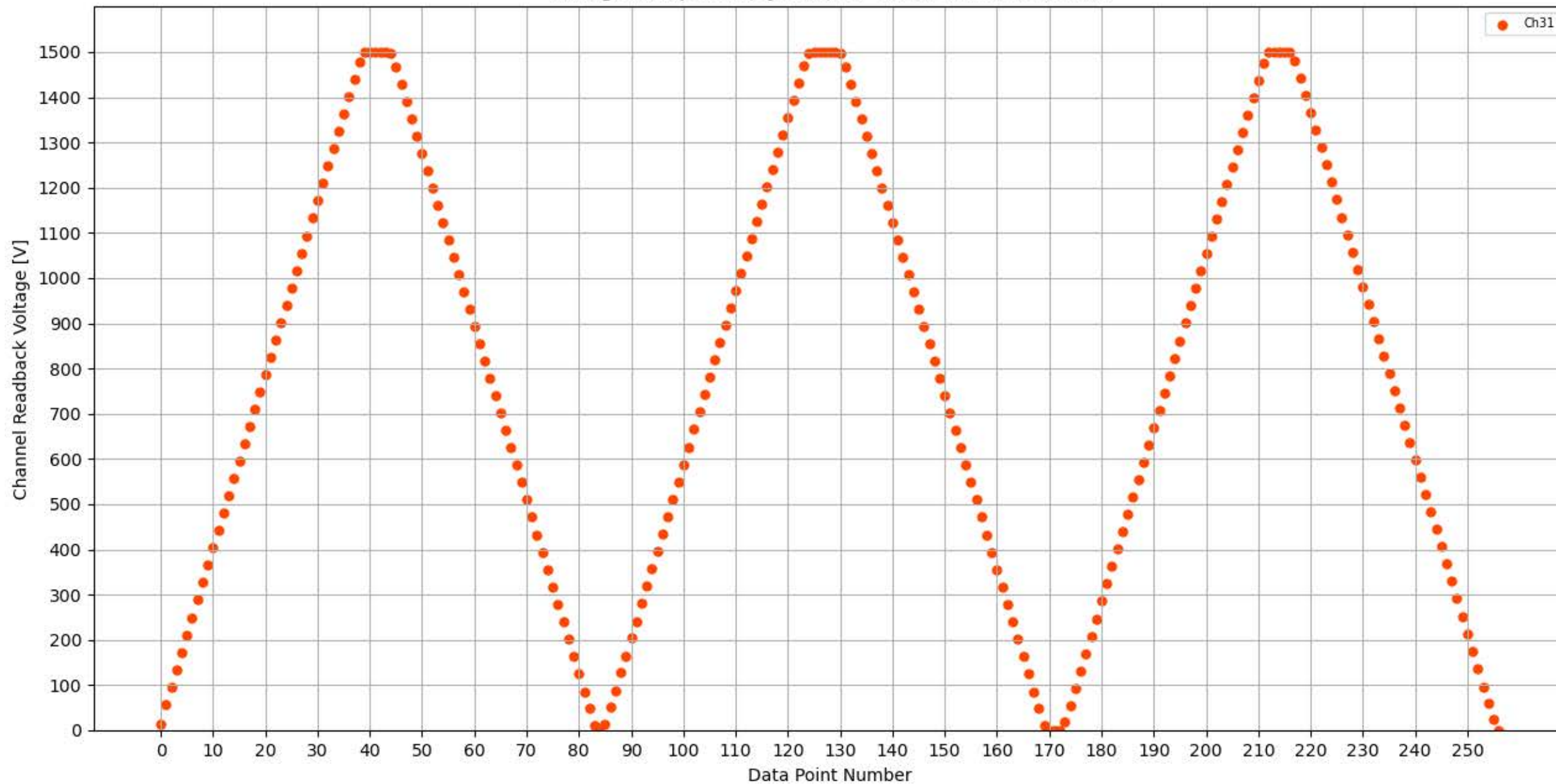
Voltage Ramp Test (Python) Bd #353, Slot #1, Ch #31
