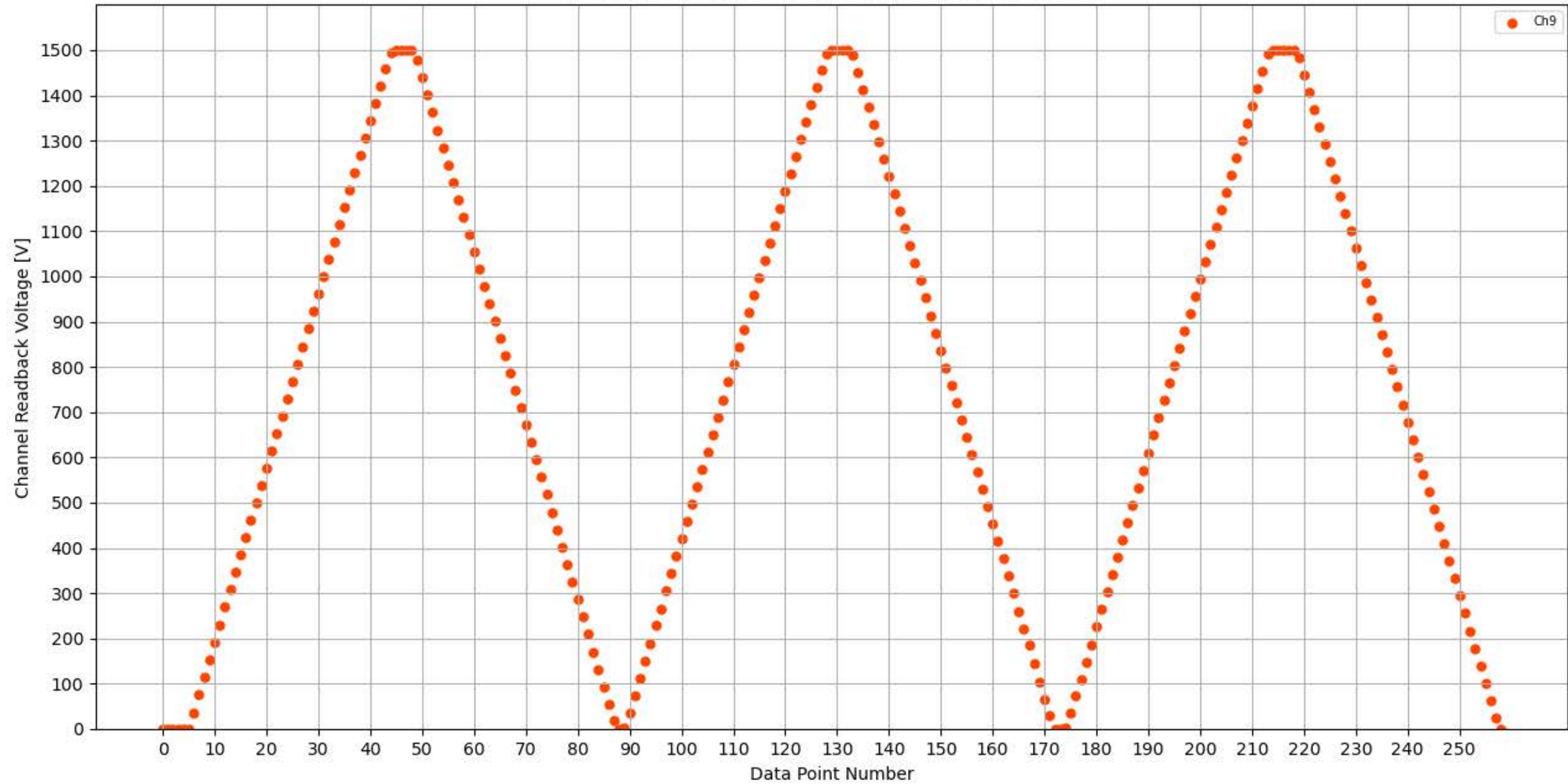
Voltage Ramp Test (Python) Bd #353, Slot #1, Ch #9
