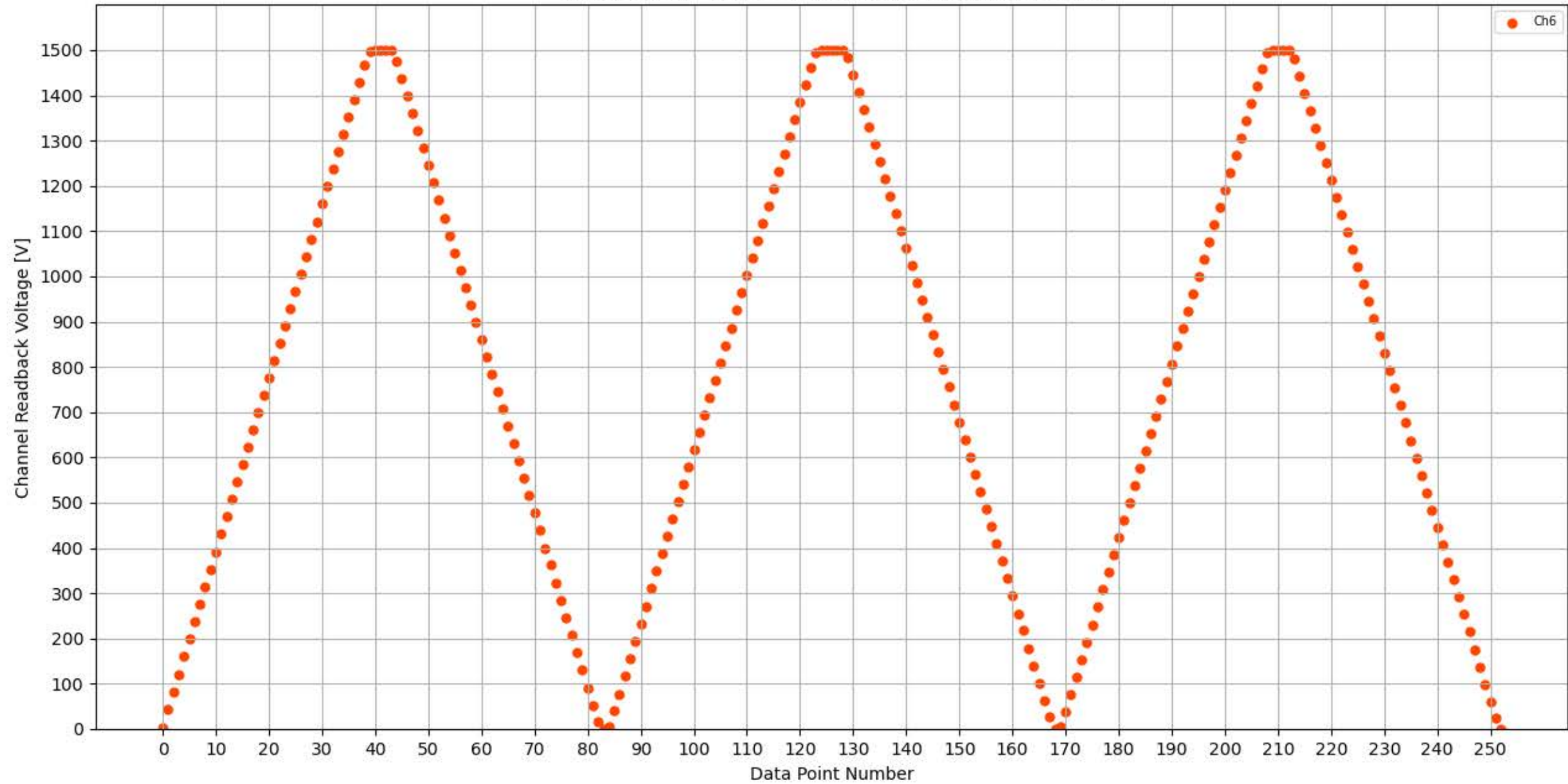
Voltage Ramp Test (Python) Bd #353, Slot #1, Ch #6
