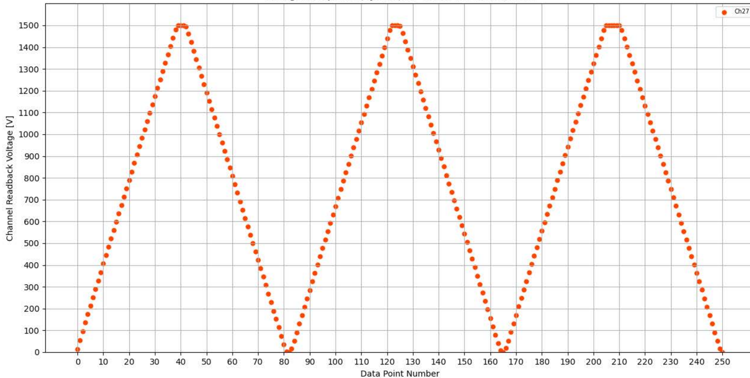
Voltage Ramp Test (Python) Bd #353, Slot #1, Ch #27
