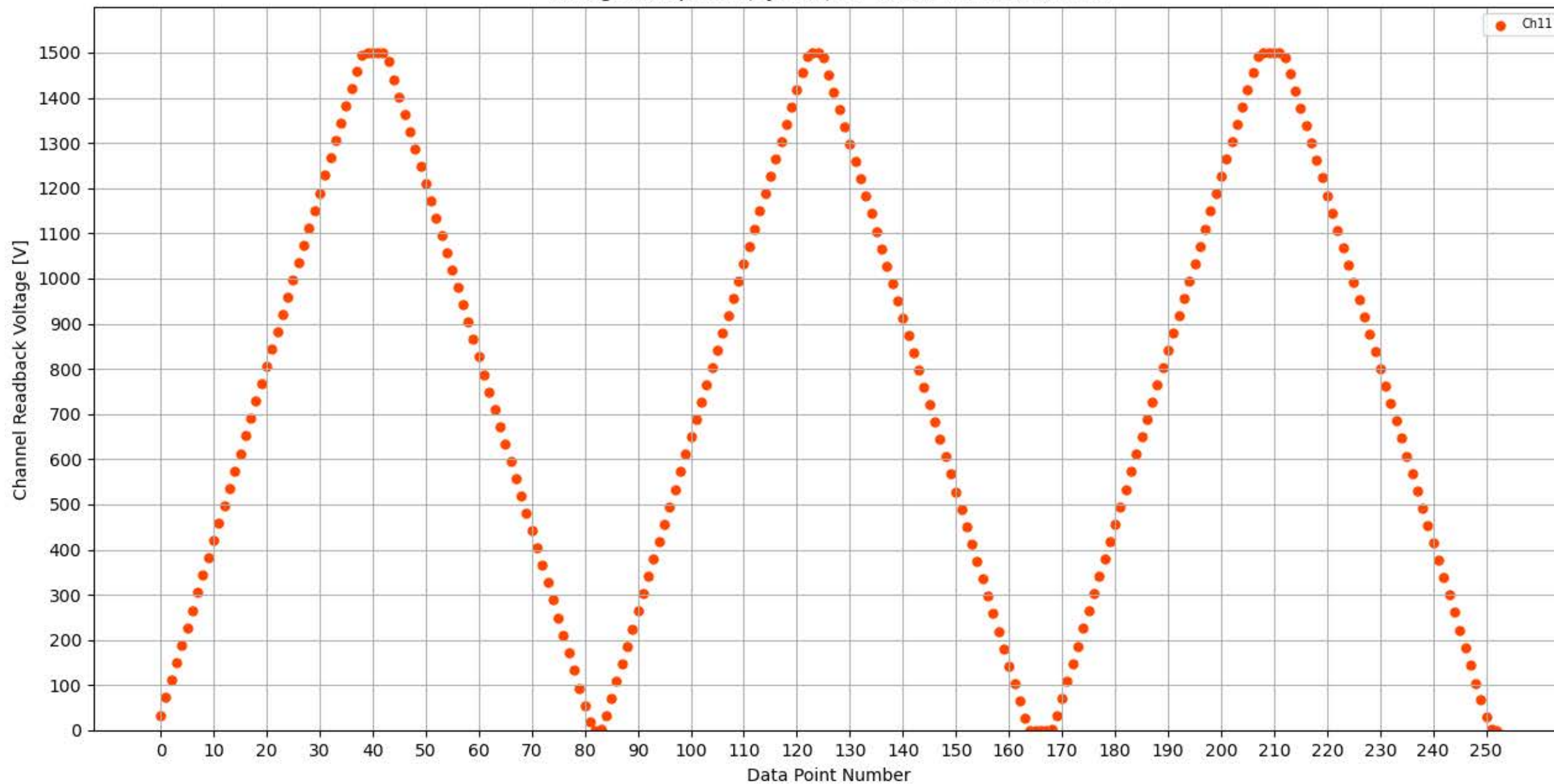
Voltage Ramp Test (Python) Bd #353, Slot #1, Ch #11
