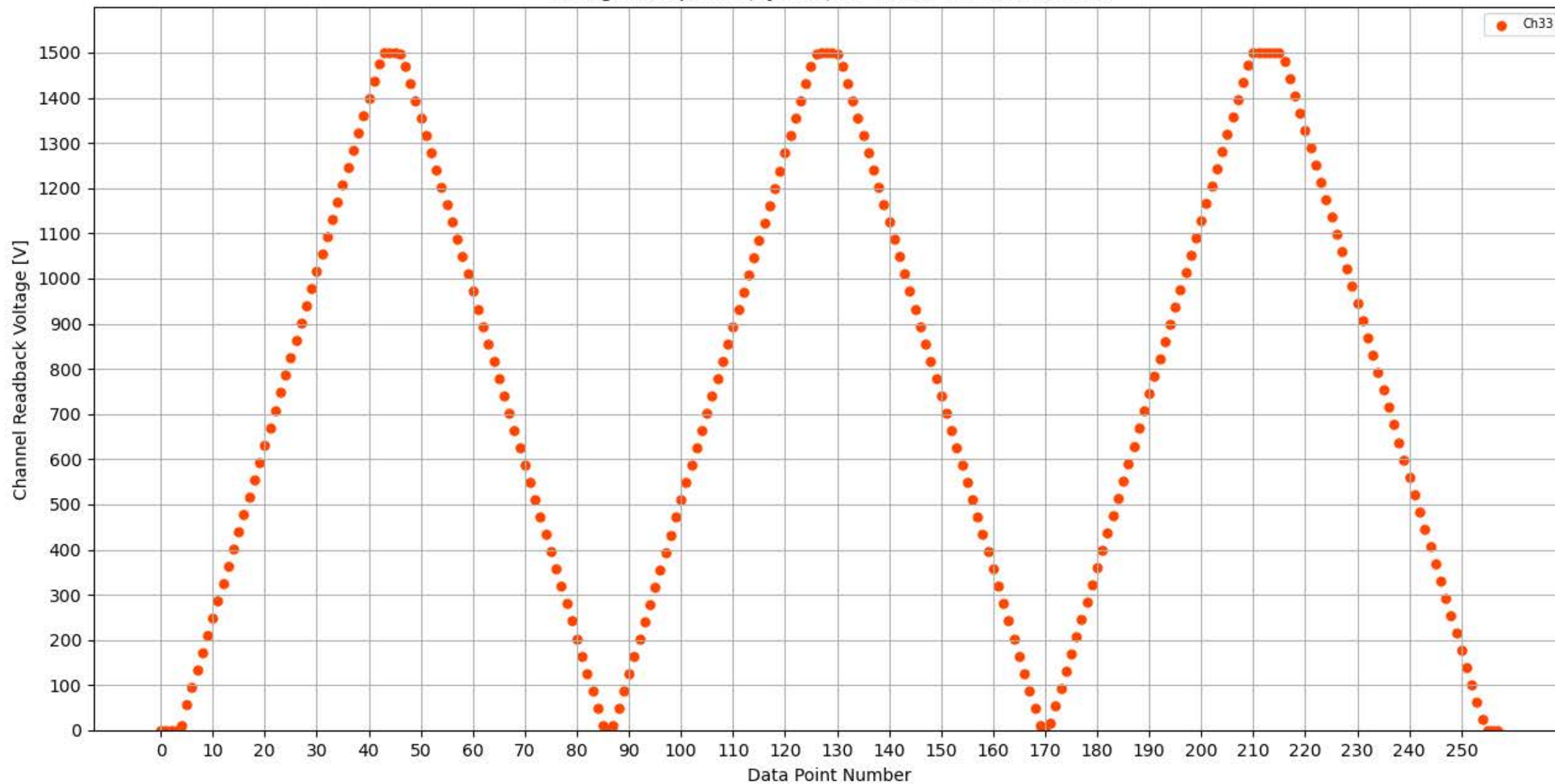
Voltage Ramp Test (Python) Bd #353, Slot #1, Ch #33
