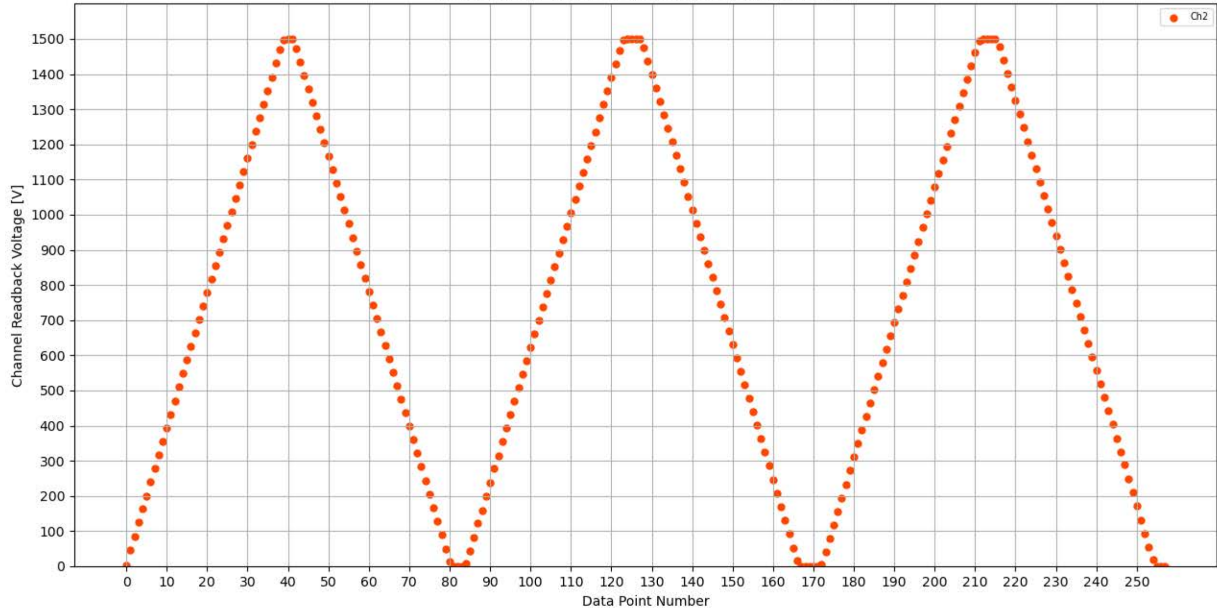
Voltage Ramp Test (Python) Bd #353, Slot #1, Ch #2
