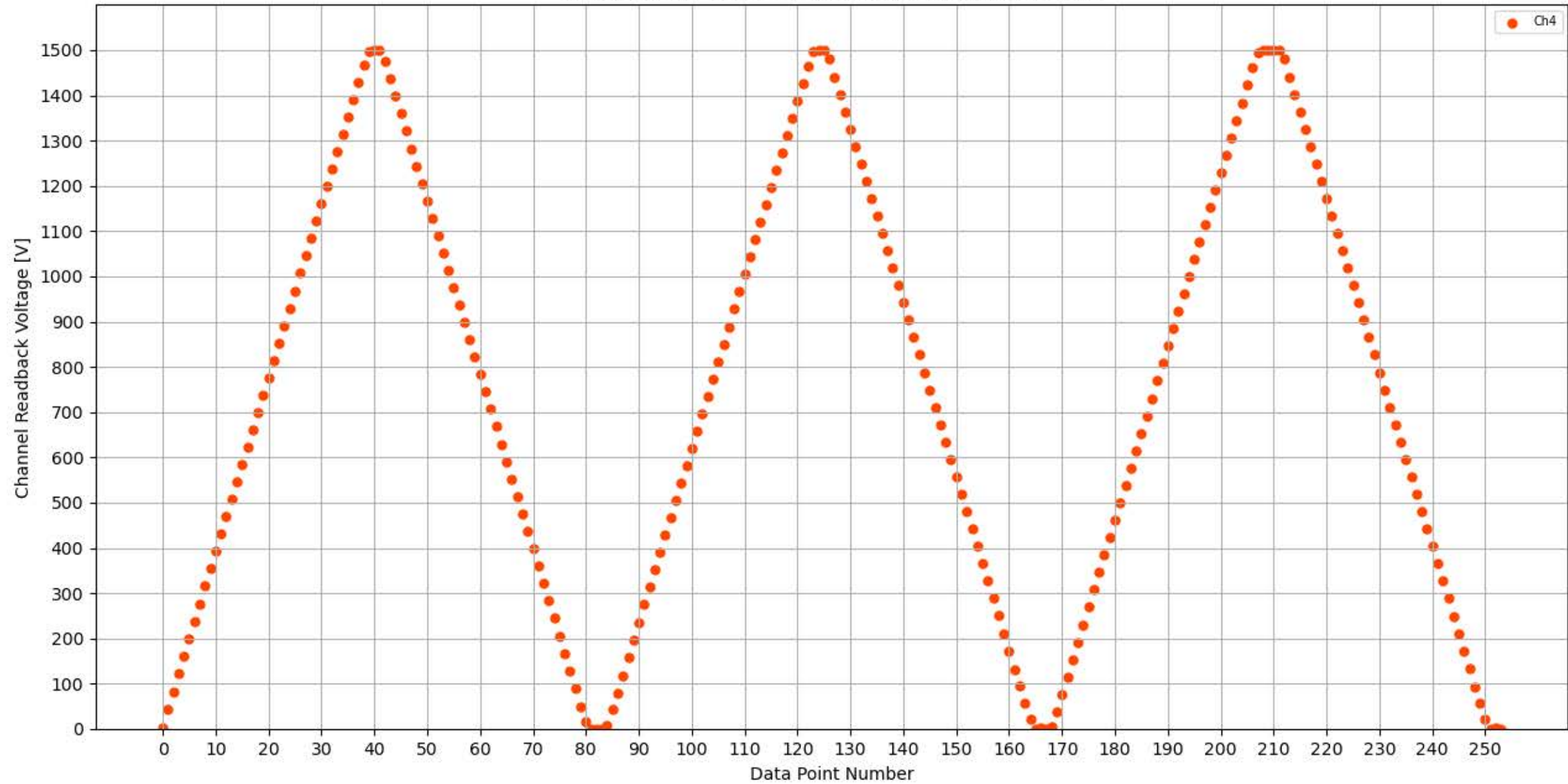
Voltage Ramp Test (Python) Bd #353, Slot #1, Ch #4
