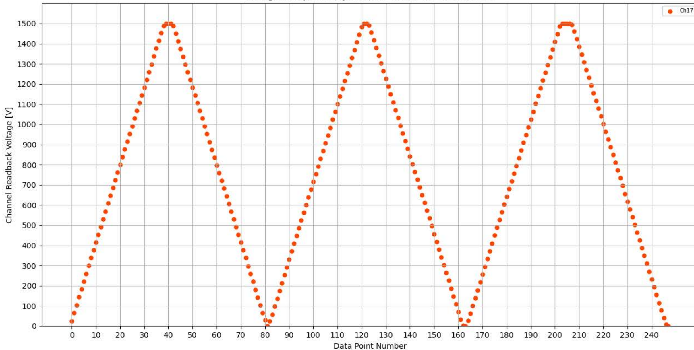
Voltage Ramp Test (Python) Bd #353, Slot #1, Ch #17
