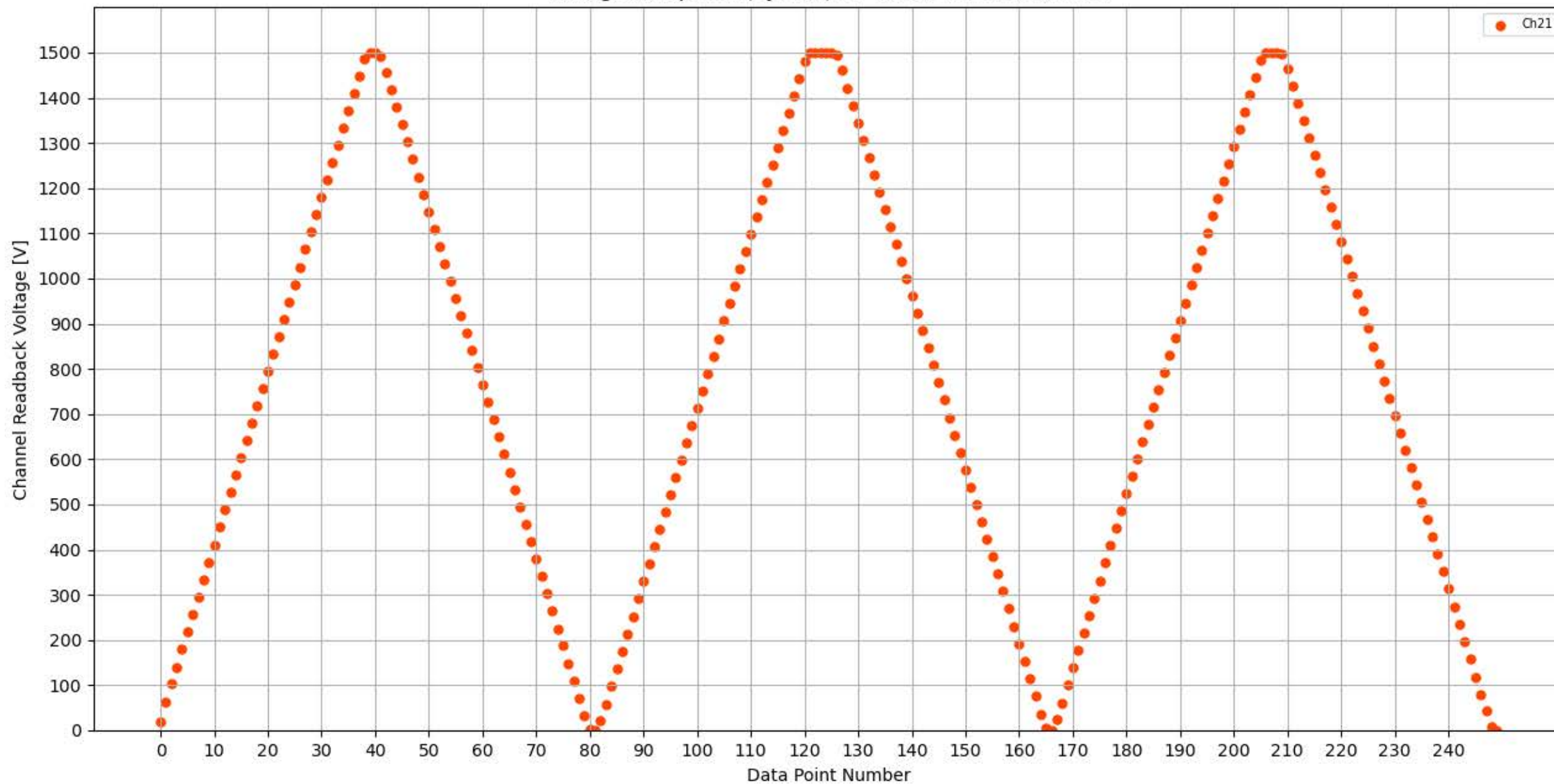
Voltage Ramp Test (Python) Bd #353, Slot #1, Ch #21
