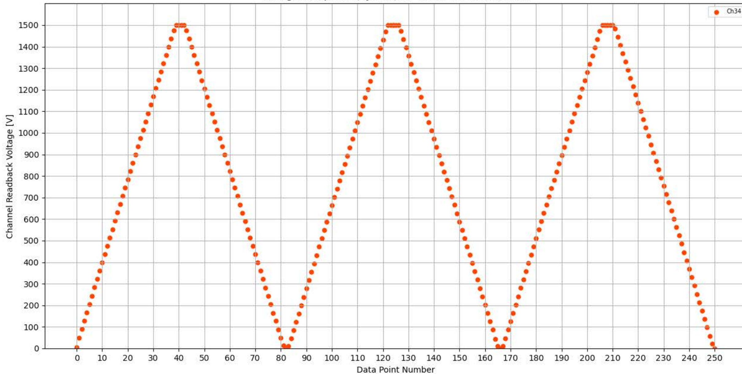
Voltage Ramp Test (Python) Bd #353, Slot #1, Ch #34
