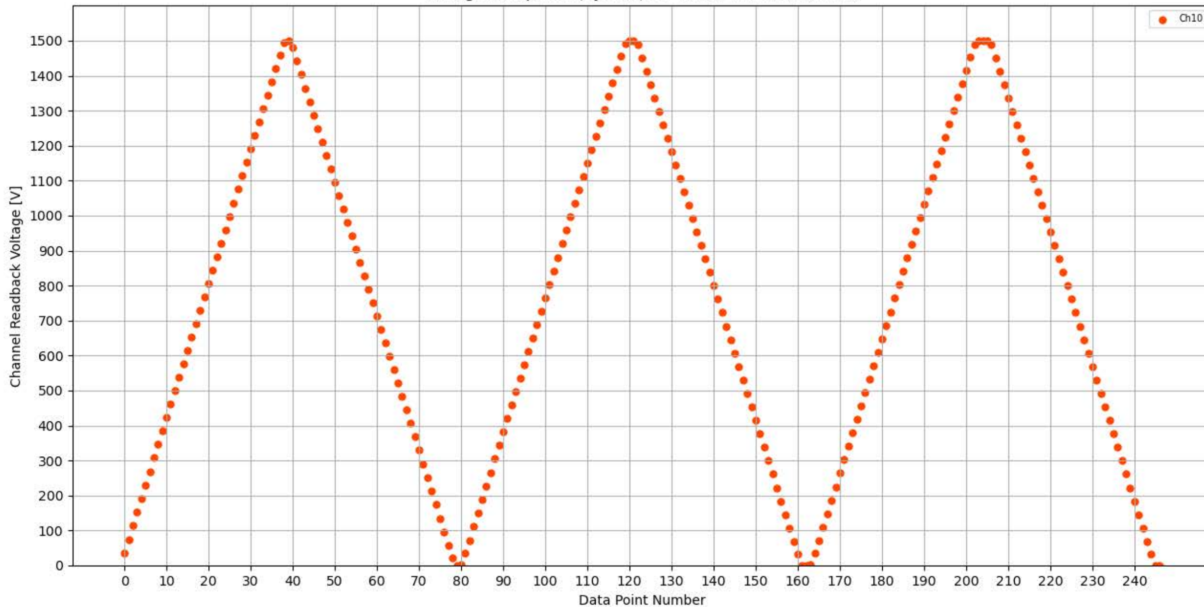
Voltage Ramp Test (Python) Bd #353, Slot #1, Ch #10
