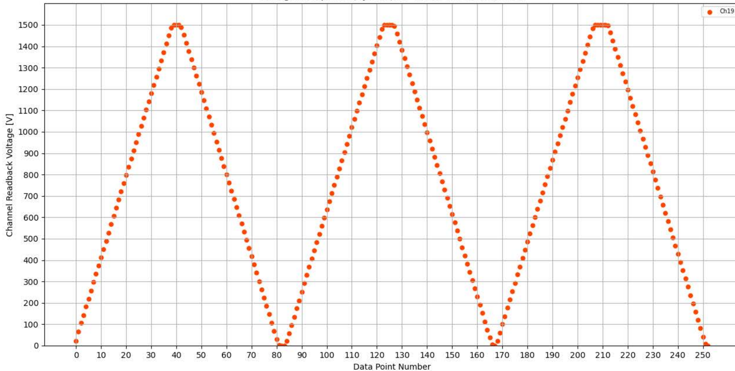
Voltage Ramp Test (Python) Bd #353, Slot #1, Ch #19
