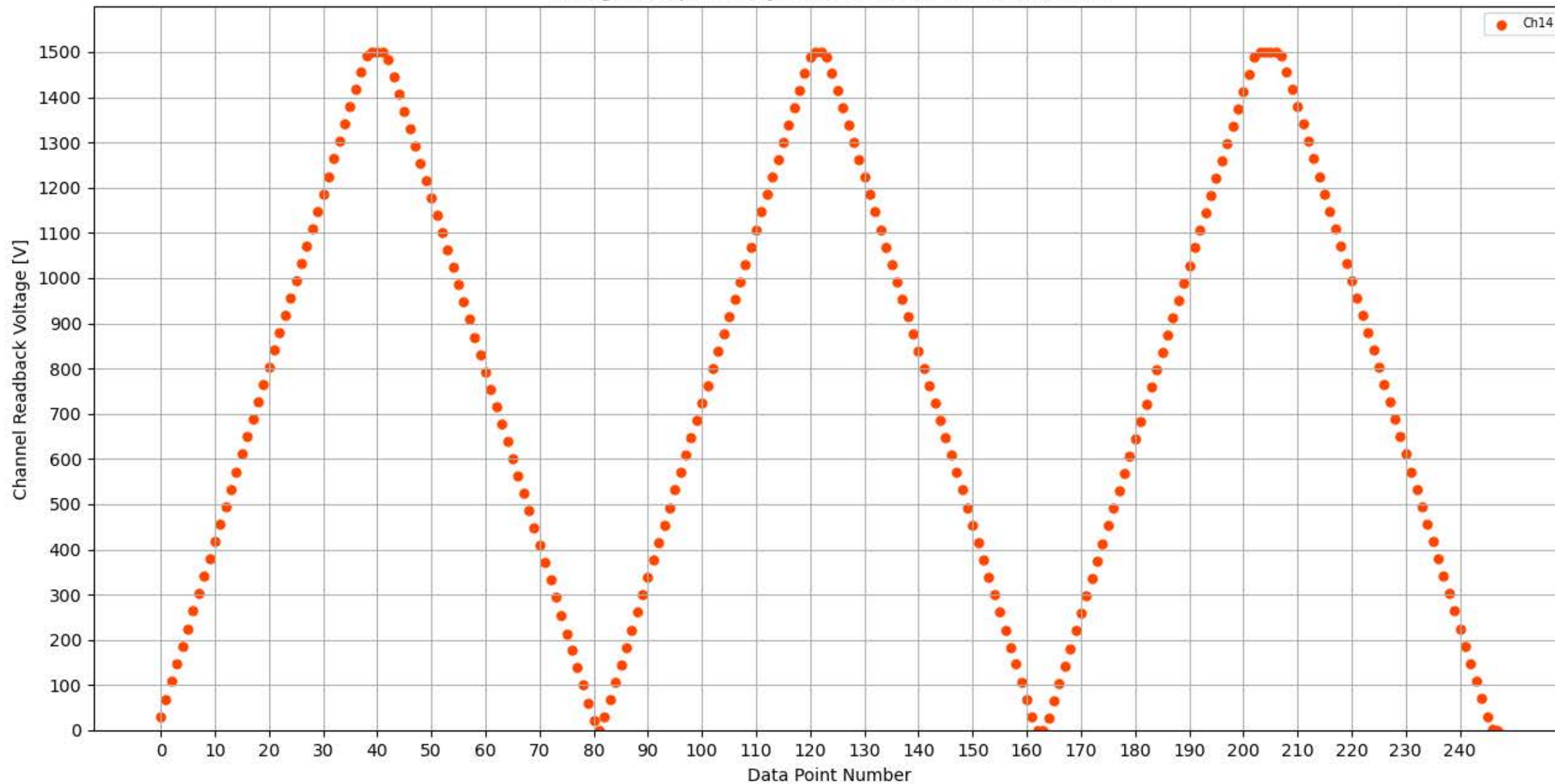
Voltage Ramp Test (Python) Bd #353, Slot #1, Ch #14
