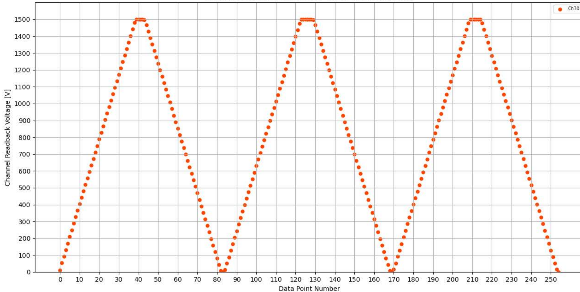
Voltage Ramp Test (Python) Bd #353, Slot #1, Ch #30
