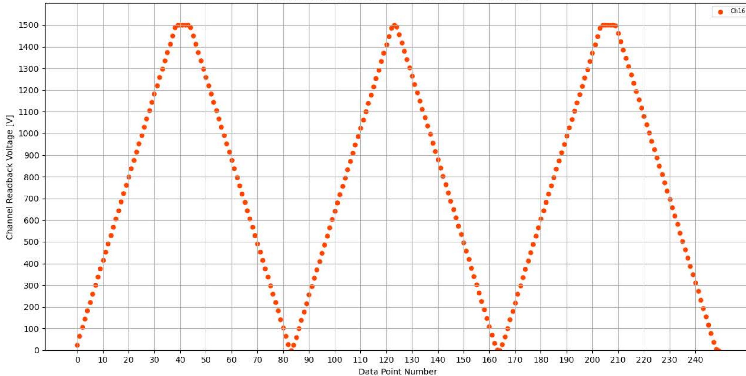
Voltage Ramp Test (Python) Bd #353, Slot #1, Ch #16
