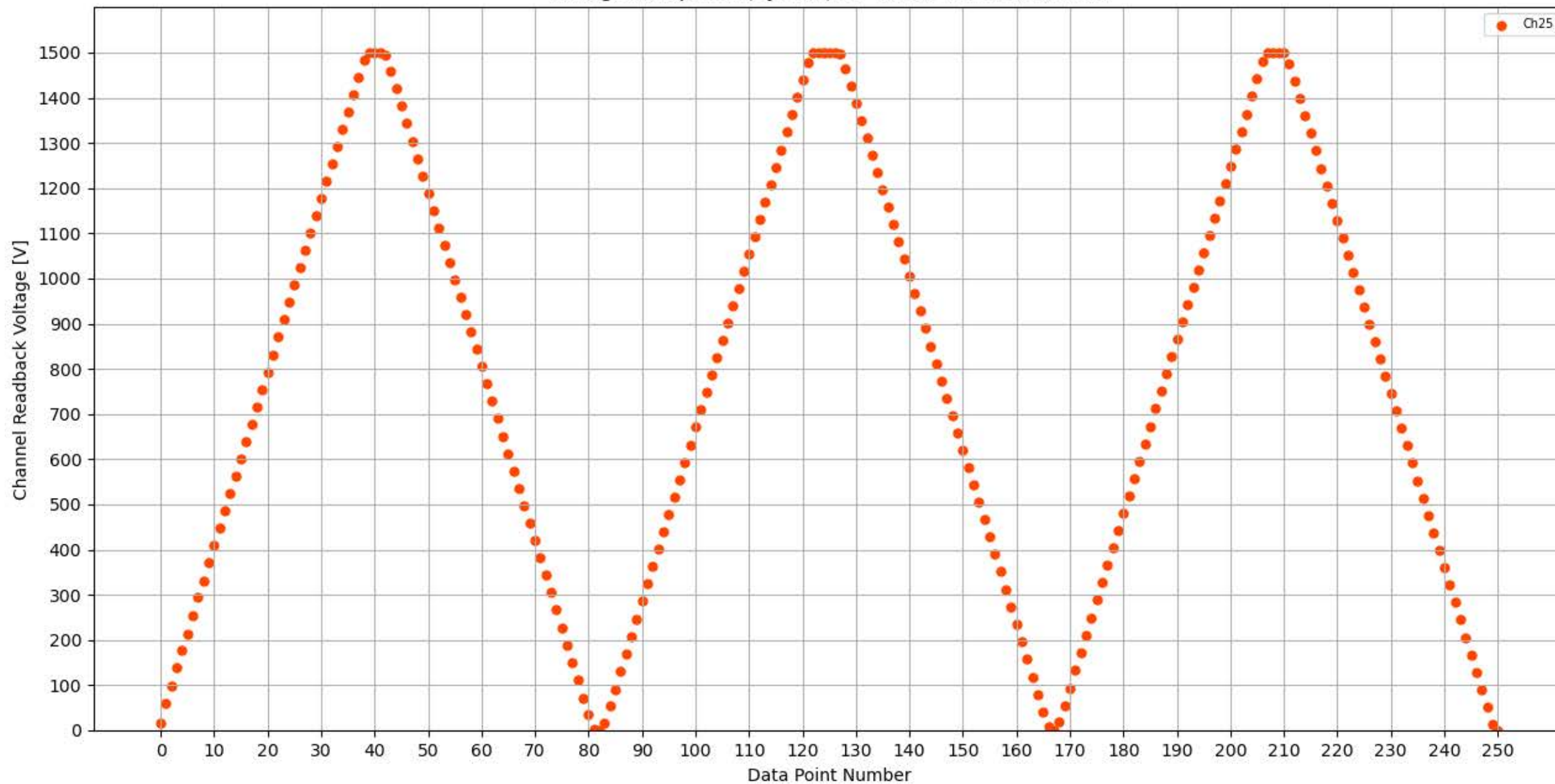
Voltage Ramp Test (Python) Bd #353, Slot #1, Ch #25
