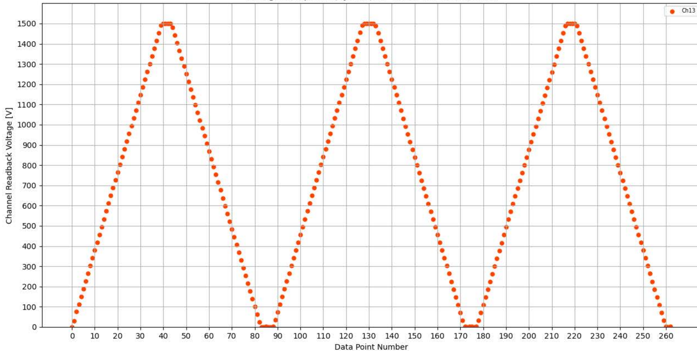
Voltage Ramp Test (Python) Bd #353, Slot #1, Ch #13
