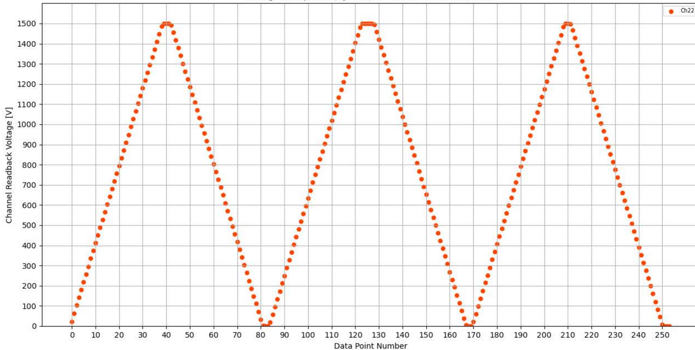
Voltage Ramp Test (Python) Bd #353, Slot #1, Ch #22
