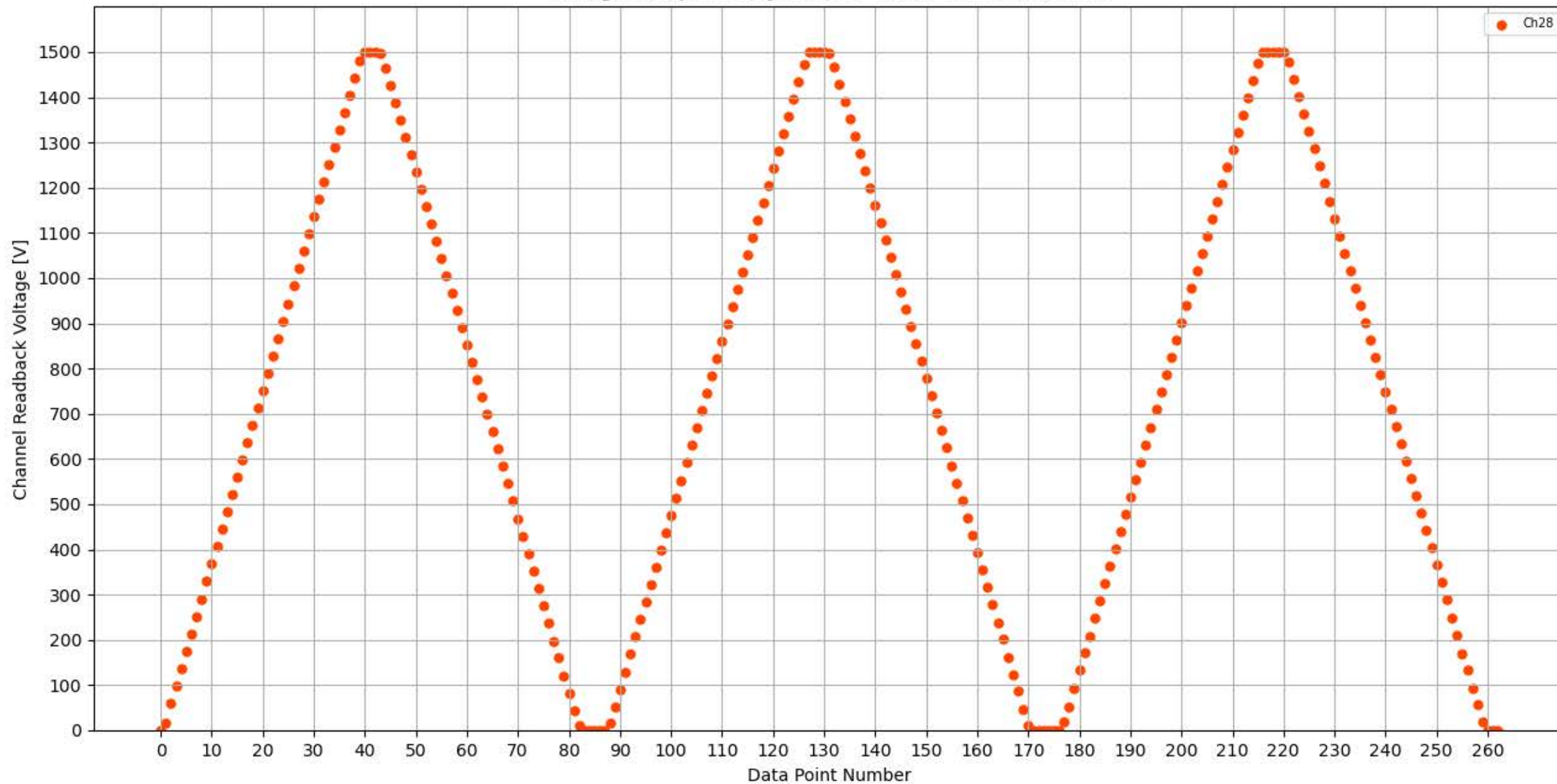
Voltage Ramp Test (Python) Bd #353, Slot #1, Ch #28
